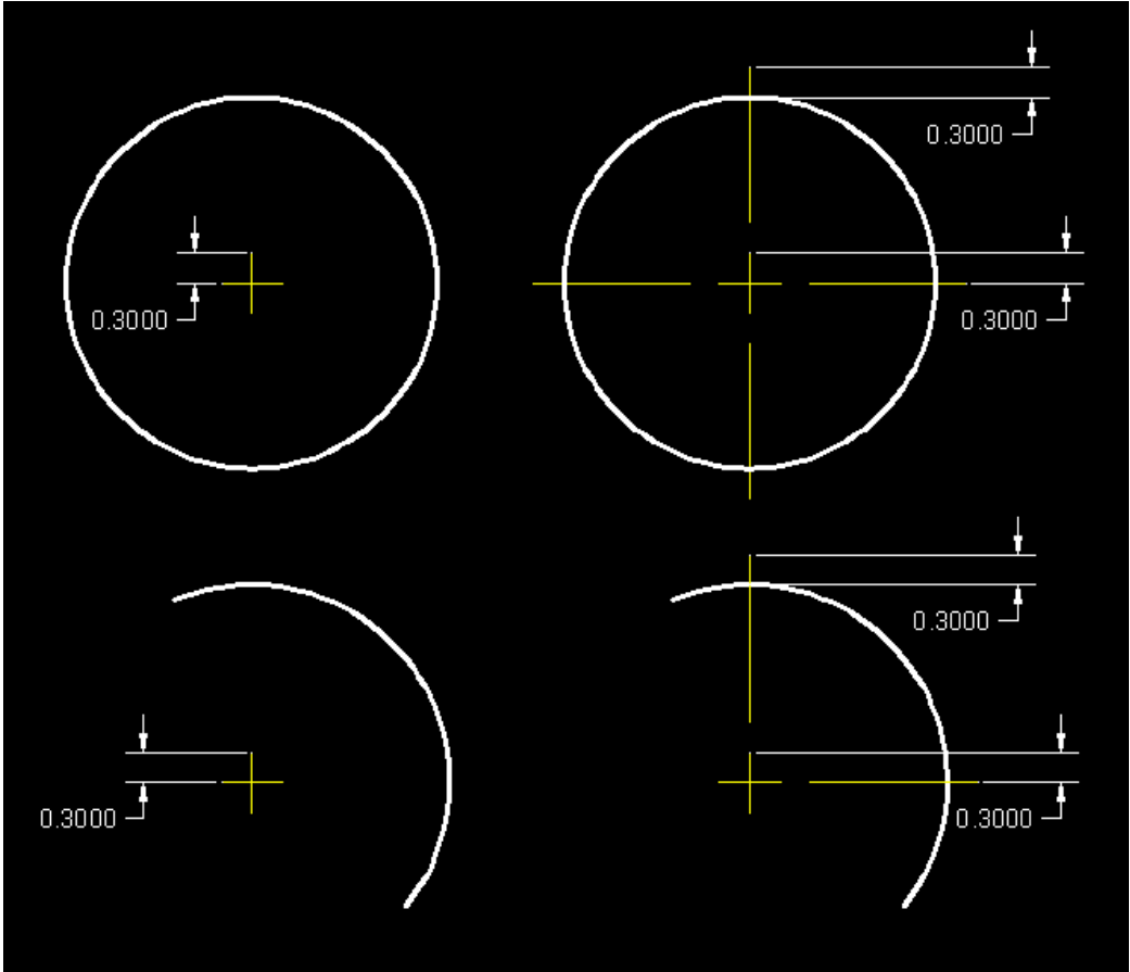
DIMCEN = 0.3
